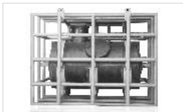
ACID TANK 3 CUBIC MTR. MOC HDPE
