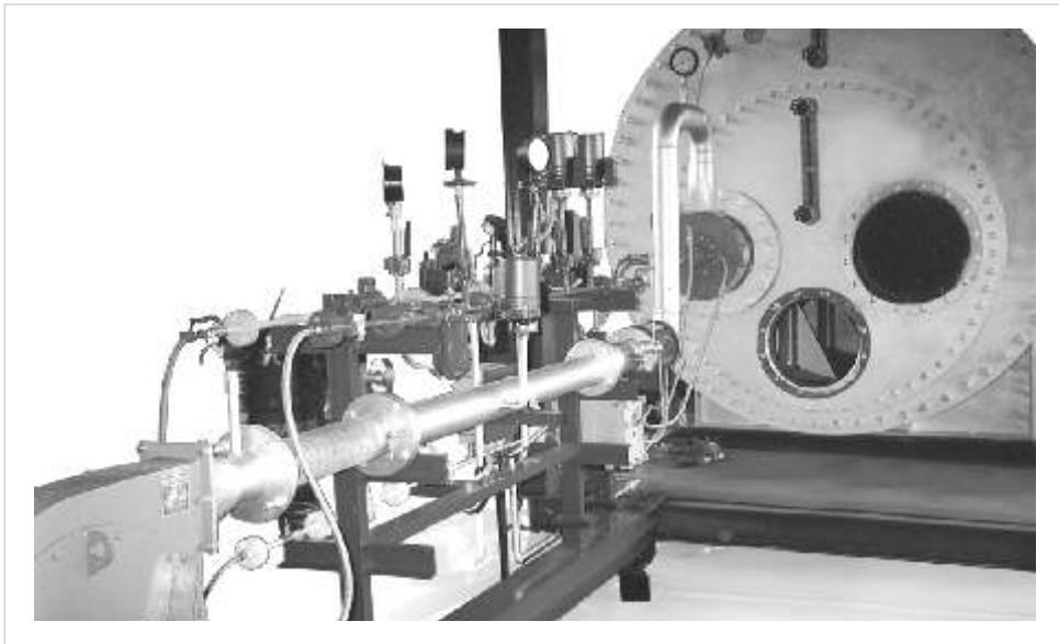
SHOP TEST OF BURNER SYSTEM WITH INDIRECT WATER BATH HEATER
